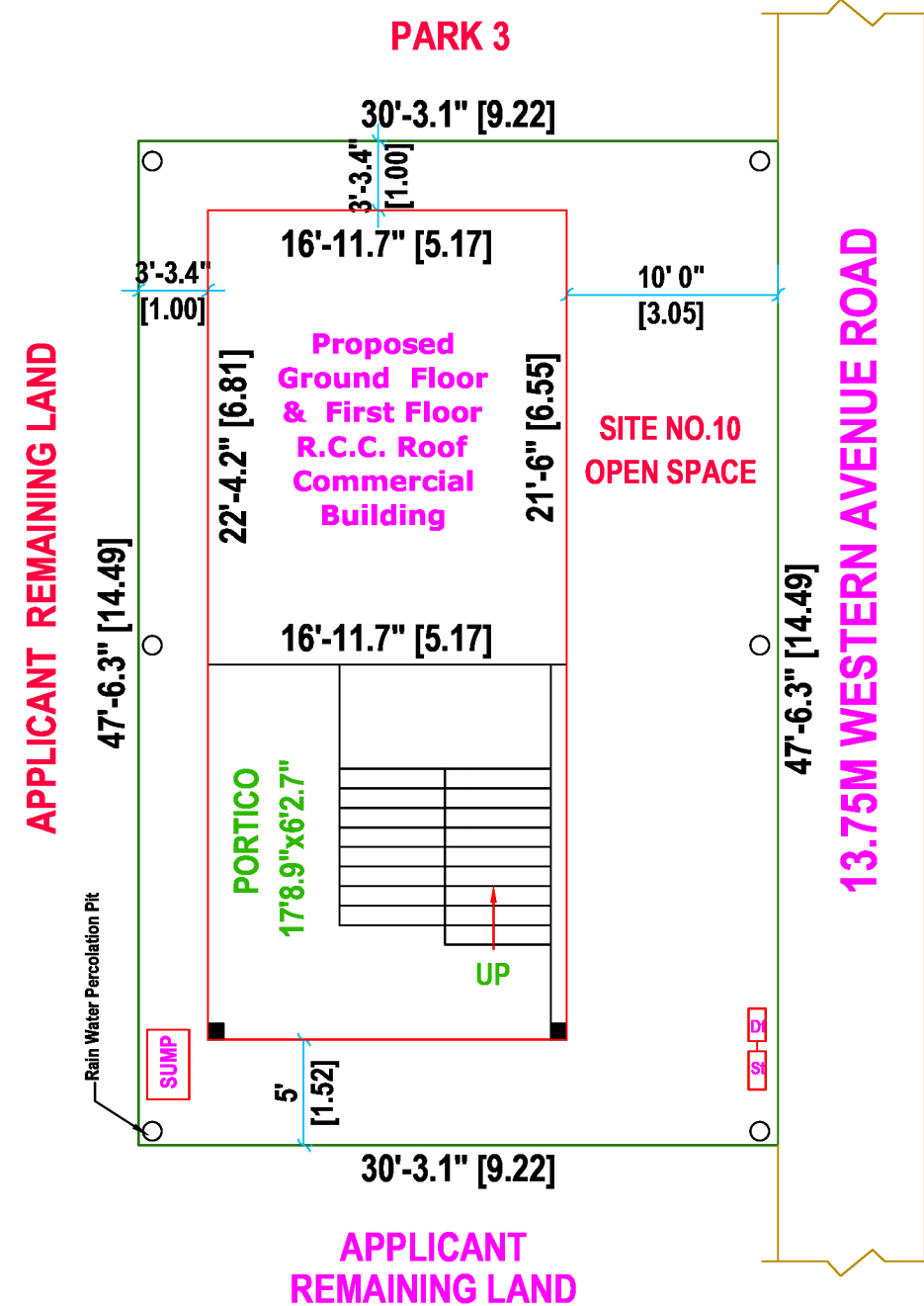
SITE PLAN SCALE 1" : 8' 0"
