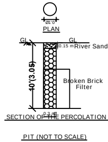
SECTION OF PERCOLATION PIT (NOT TO SCALE)
