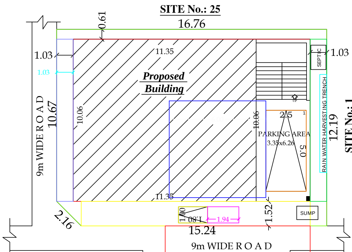
SITE PLAN
