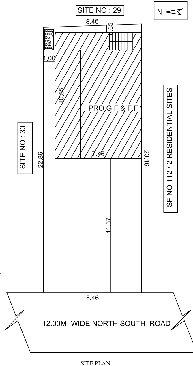
SITE PLAN
