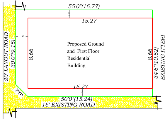
SITE PLAN
