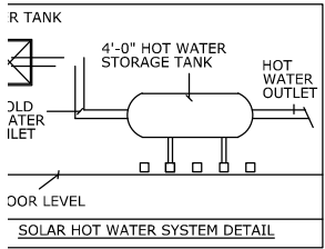
SOLAR HOT WATER SYSTEM DETAIL
