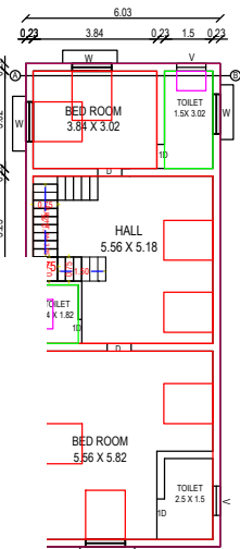
PROPOSED FIRST FLOOR BUILDING
