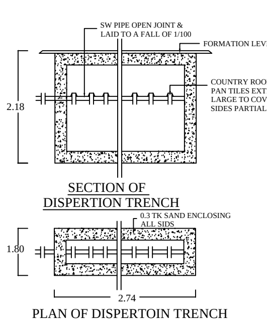
DISPERSION TRENCH
