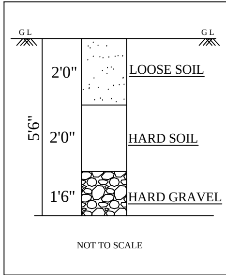
TRIAL PIT
