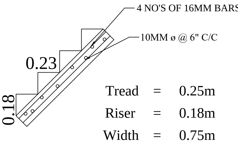
STAIRCASE DETAILS
