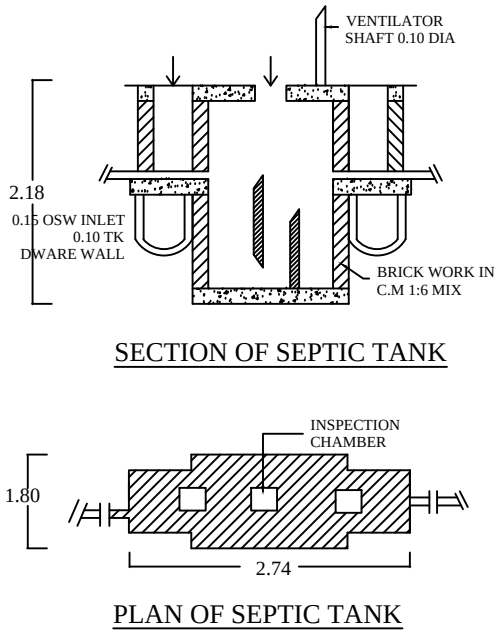
SEPTIC TANK
