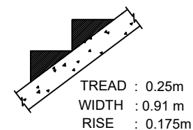
STAIRCASE DETAIL:
