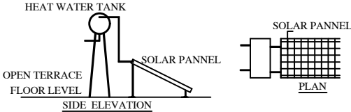
SOLAR WATER HEATER (NOT TO SCALE)
