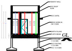
SECTION AB
