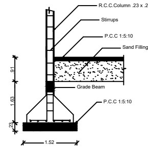
COLUMN DETAIL
