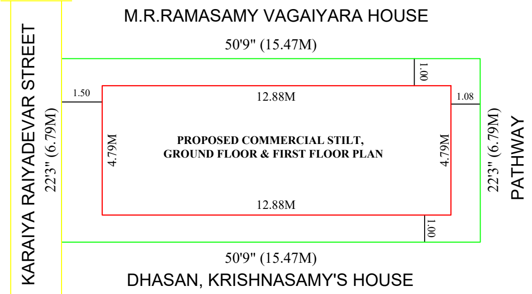
SITE PLAN
