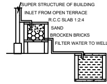
RAINWATER HARVESTING
