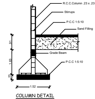
COLUMN DETAIL
