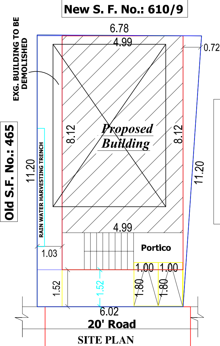
SITE PLAN
