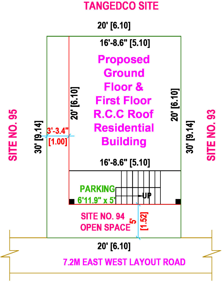
SITE PLAN (SCALE - 1" : 8' 0")
