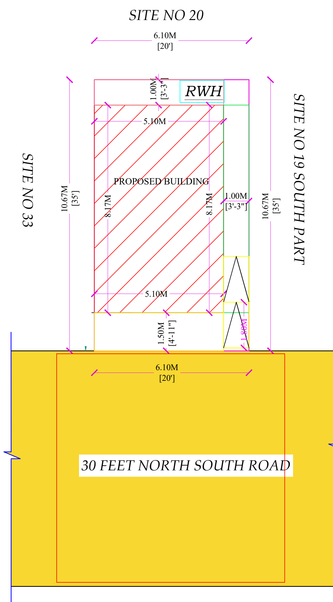
SITE PLAN Site Plan (Scale 1"=8'0")
