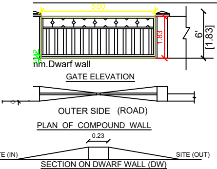
SECTION ON DWARF WALL (DW)
