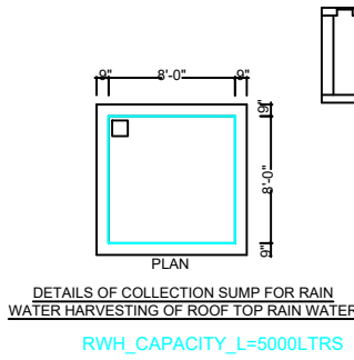
RWH_CAPACITY_L=5000LTRS
