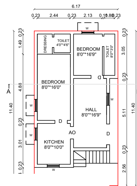
R PLAN
