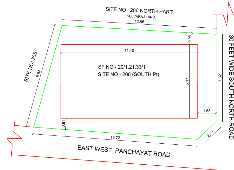
SITE PLAN
