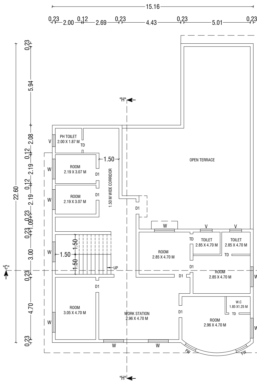
BLOCK - 03 - DORMITORIES_FIRST FLOOR PLAN
