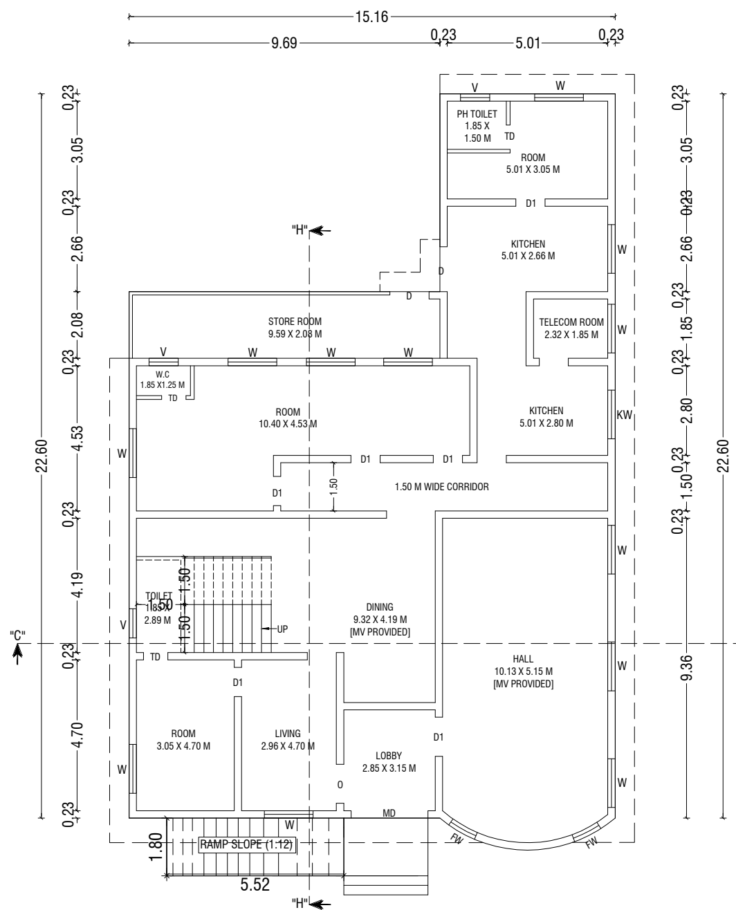
BLOCK - 03 - DORMITORIES_GROUND FLOOR PLAN
