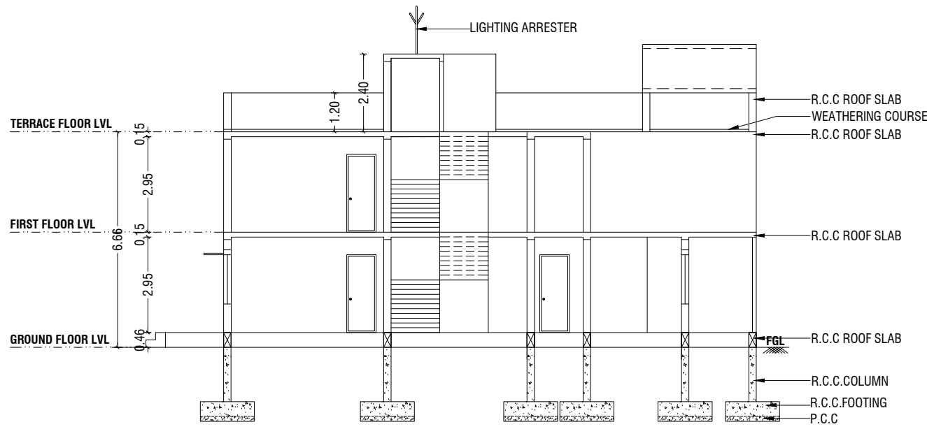
BLOCK - 03_SECTION "HH" @ WEST SIDE
