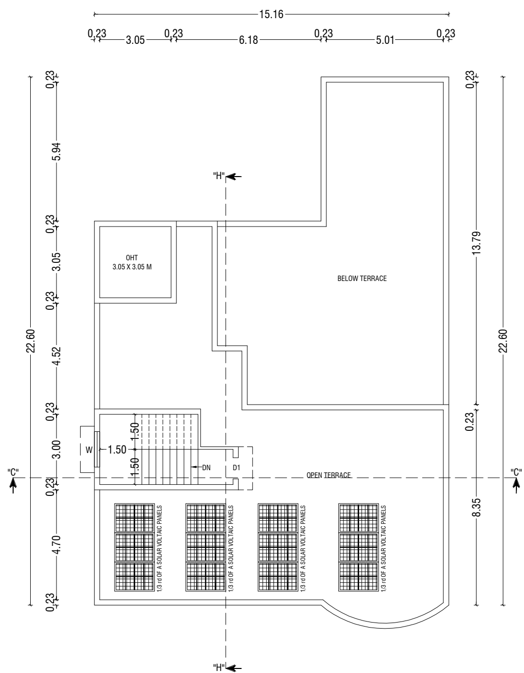
BLOCK - 03 - DORMITORIES_TERRACE FLOOR PLAN
