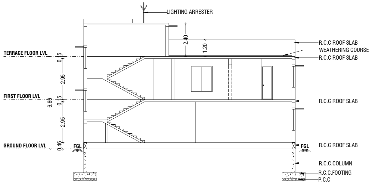
BLOCK - 03_SECTION "CC" @ NORTH SIDE
