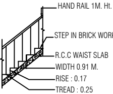
STAIR DETAIL
