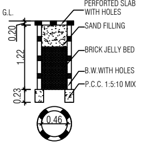
RAIN WATER HARVEST
