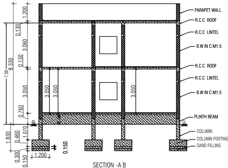
SECTION - A B
