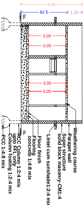
SECTION ELEVATION
