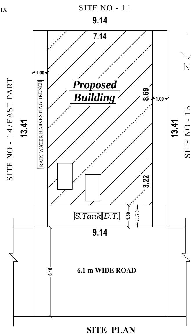
SITE PLAN
