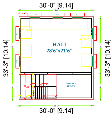
PROPOSED GROUND FLOOR PLAN
