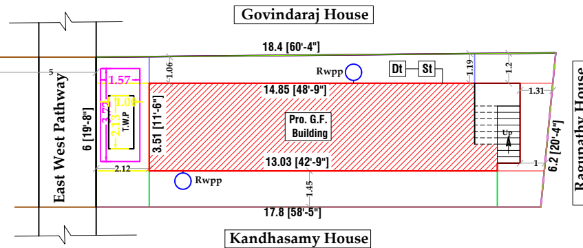
LOCATION PLAN
