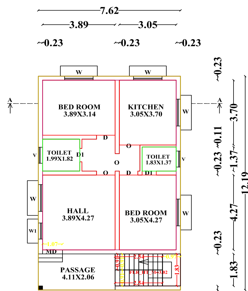
TYPICAL_FLOOR_PLAN=1,2 TYPICAL FIRST FLOOR PLAN AND SECOND FLOOR PLAN
