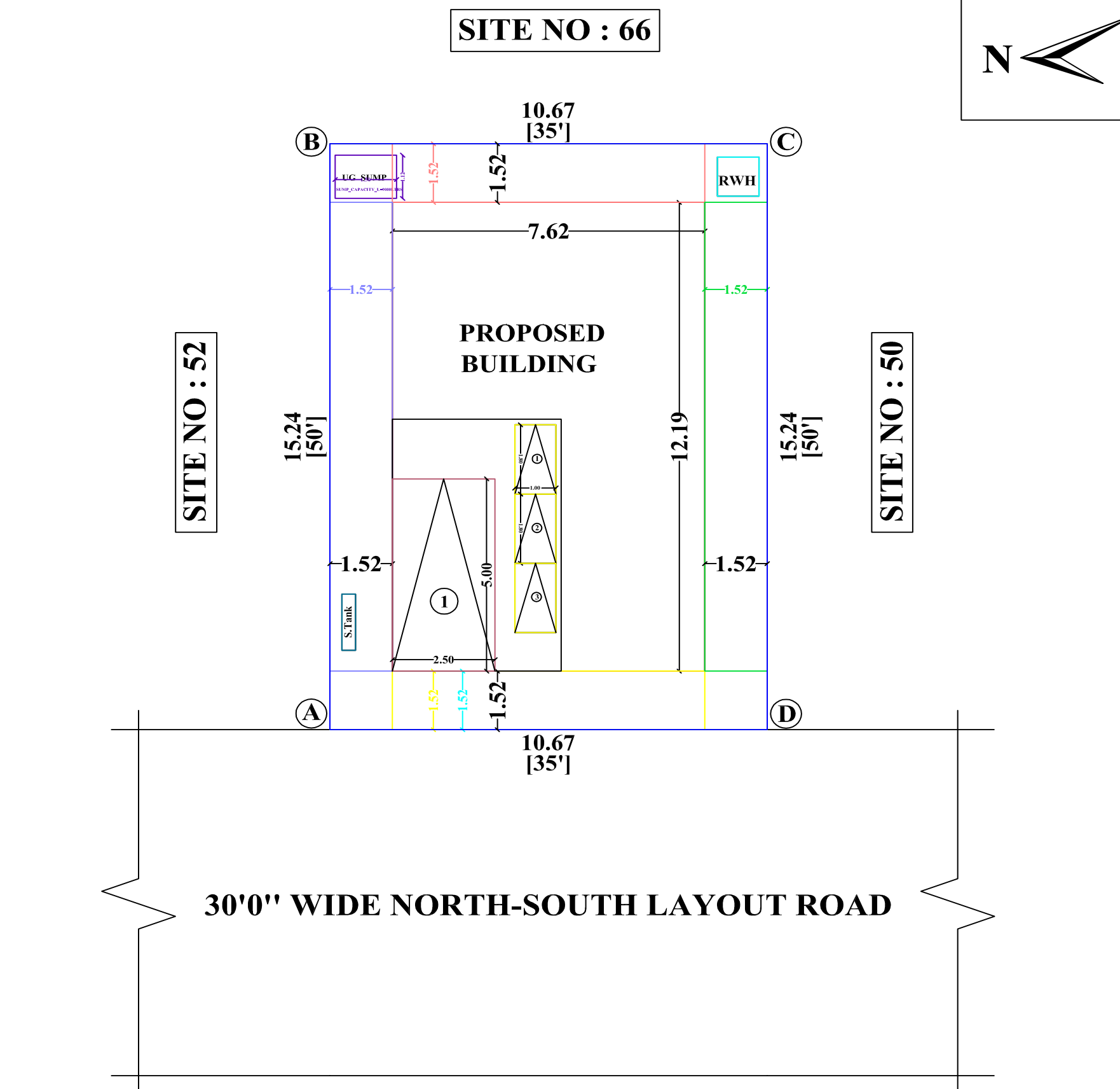
SITE PLAN
