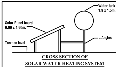
CROSS SECTION OF SOLAR WATER HEATING SYSTEM
