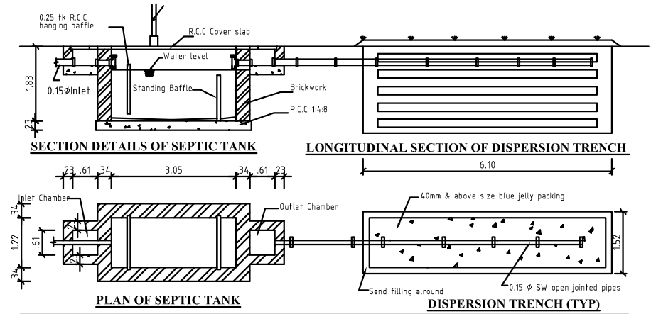
DETAILS OF SEPTIC TANK - 250 GALLONS & DISPERSION TRENCH
