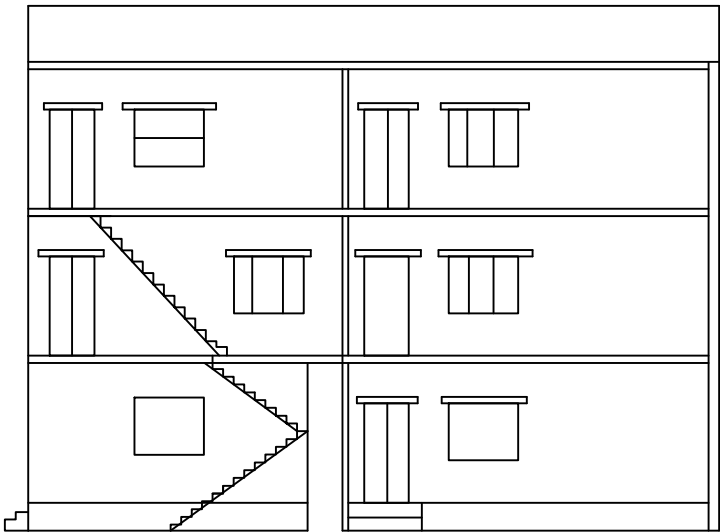
NORTH FACE ELEVATION
