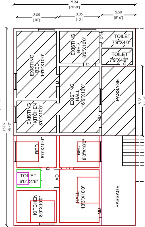
EXISTING FIRST FLOOR AND PRO.ADDITIONAL FIRST FLOOR
