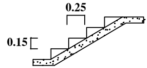
STAIR CASE DETAILS: (Not to Scale)
