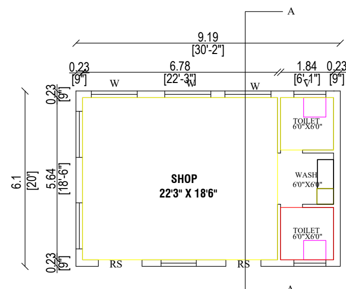
PROPOSED GROUND FLOOR
