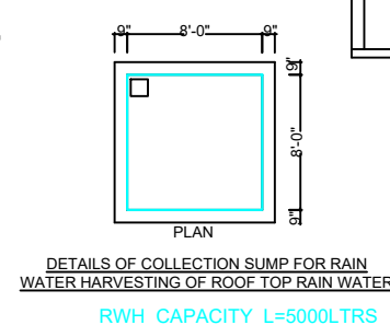
RW_H_CAPACITY_L=5000LTRS
