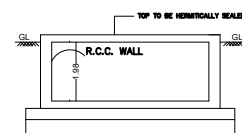
RWH SECTION (SAMPLE) RWH_CAPACITY_L=2000LTRS
