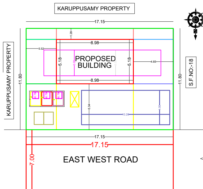
SITE PLAN
