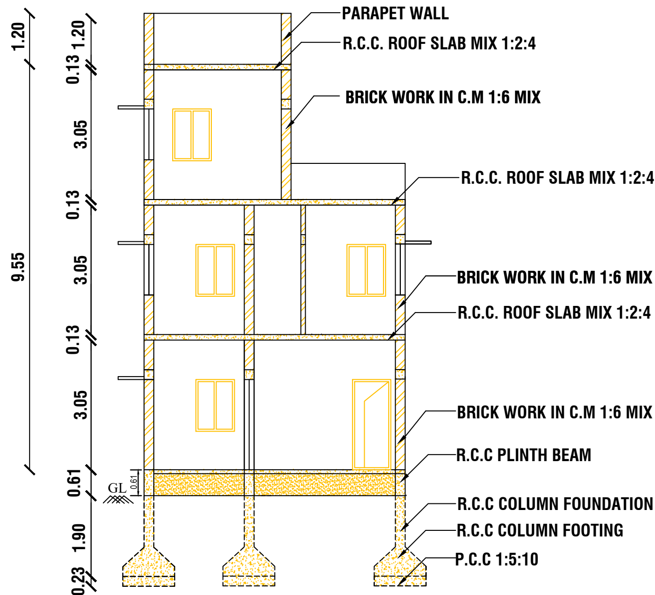
CROSS SECTION AT A-A
