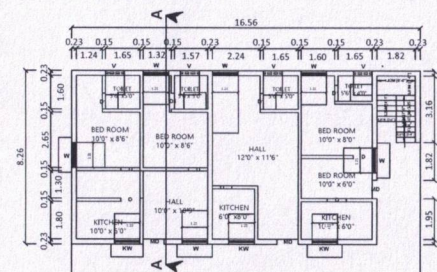
PRO.SECOND FLOOR
