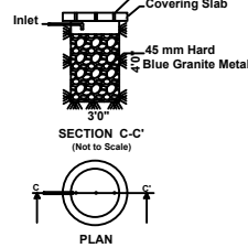
Rain Water Percolation Pit (Not to Scale)
