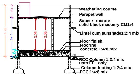
SECTION ELEVATION
