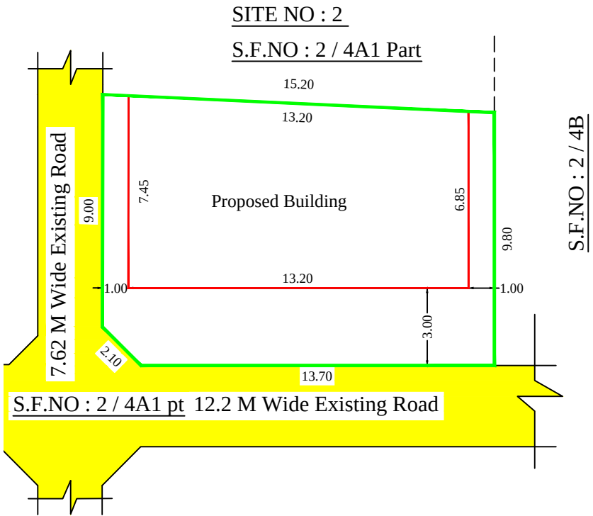
SITE PLAN
