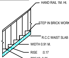
STAIR DETAIL
