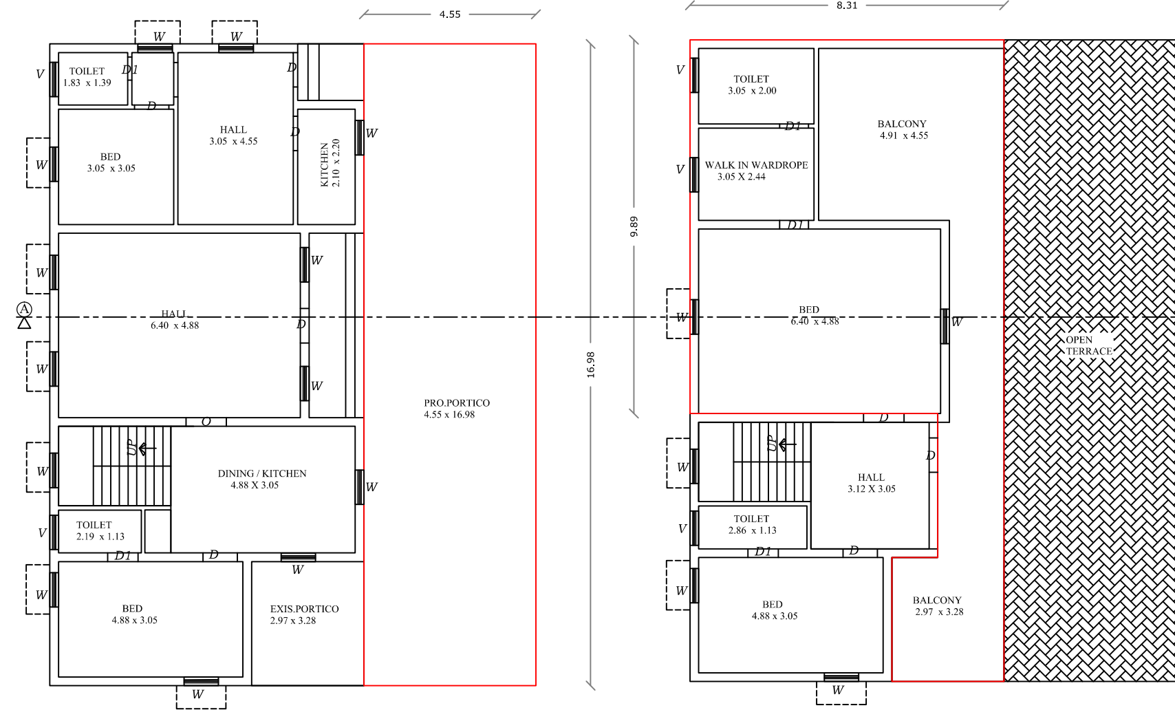
EXISTING & PROPOSED GROUND FLOOR PLAN
