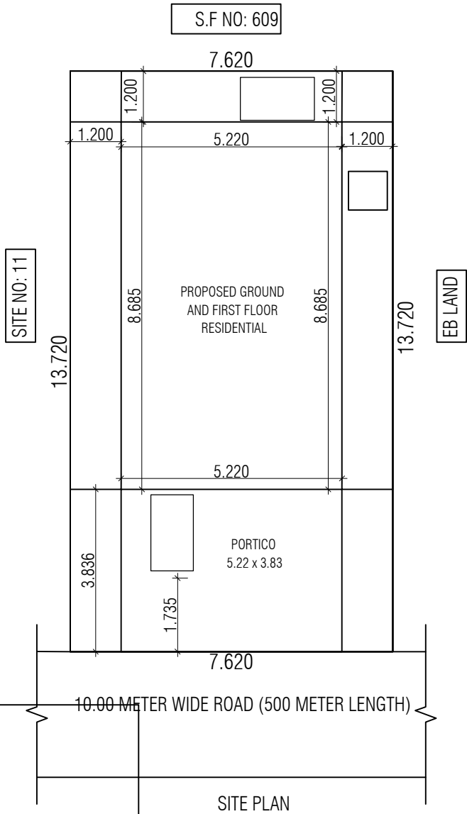
SITE PLAN
