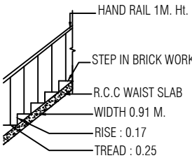
STAIR DETAIL
