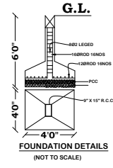
EARTHQUAKE SAFE DESIGN (NOT TO SCALE)
