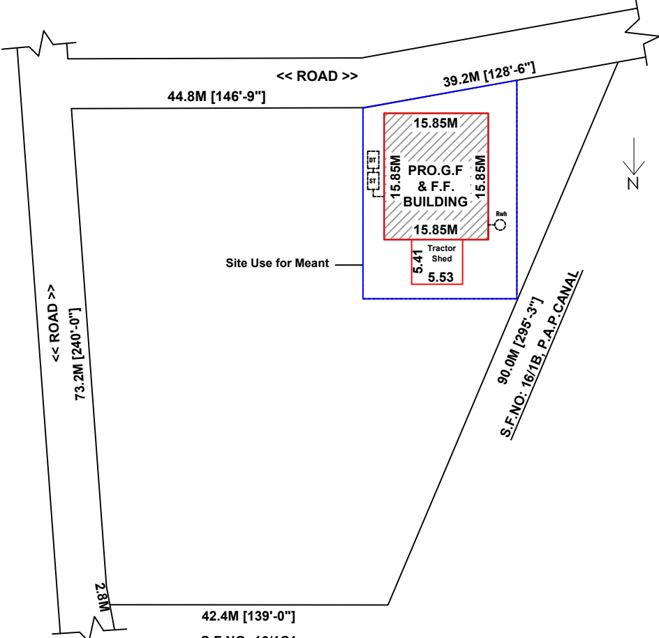
SITE PLAN
