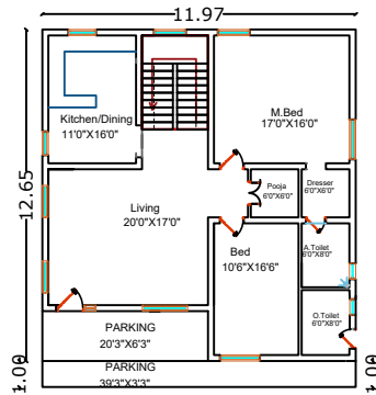
PRO. G.F. BUILDING PLAN
