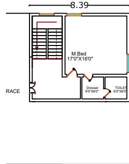
EXISTED. F.F. BUILDING PLAN
