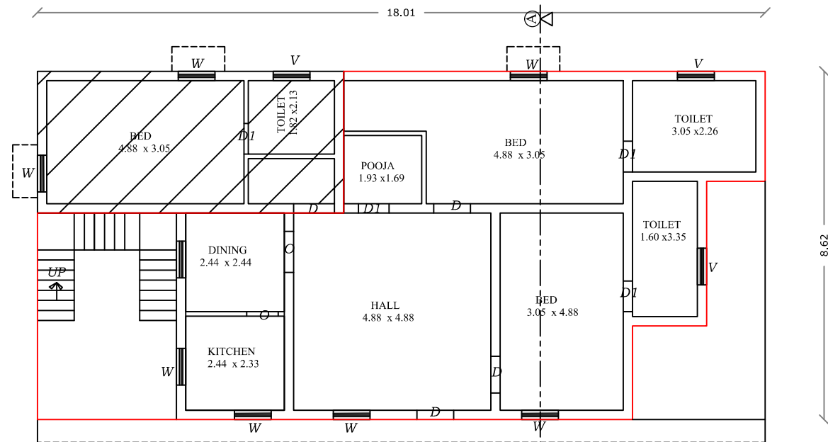
EXISTING & PROPOSED FIRST FLOOR PLAN
