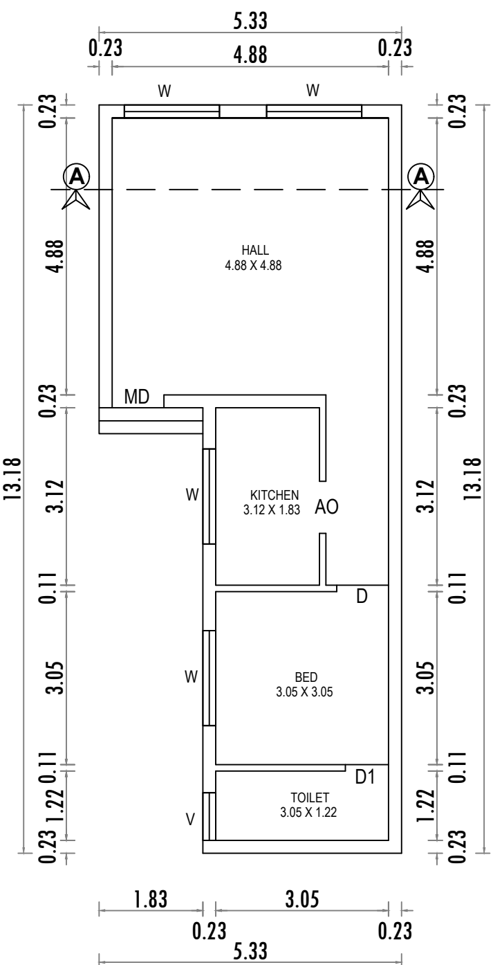
FLOOR PLAN
