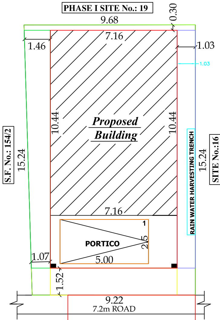
SITE PLAN
