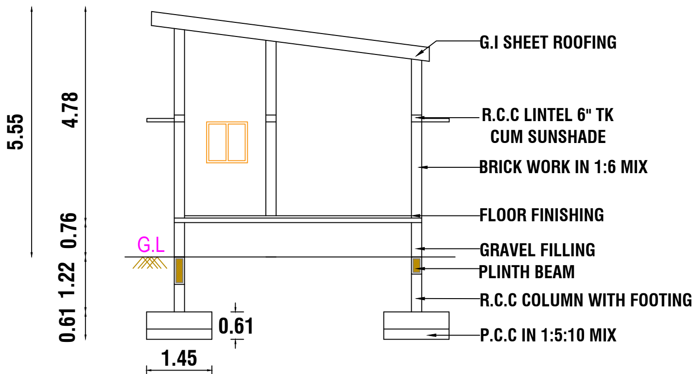
CROSS SECTION AT A-A
