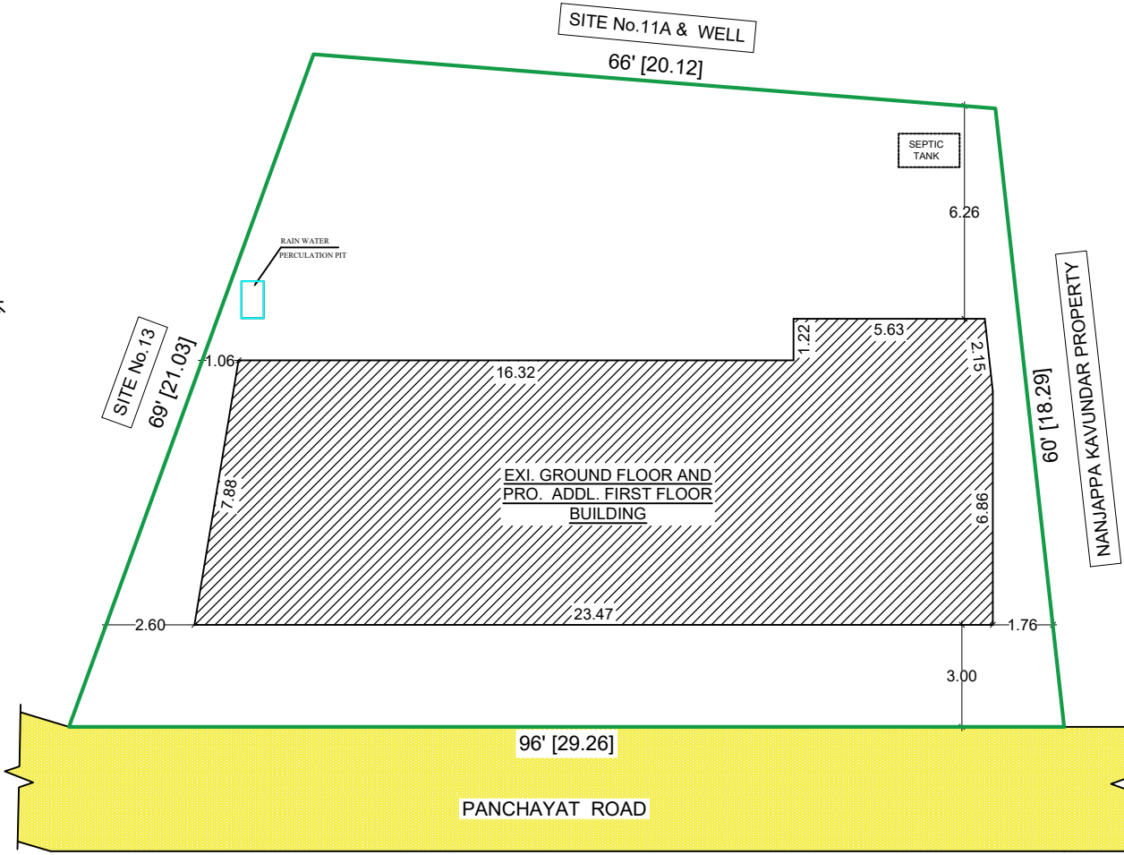
SITE PLAN
