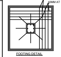
FOOTING DETAIL SCALE: NTS
