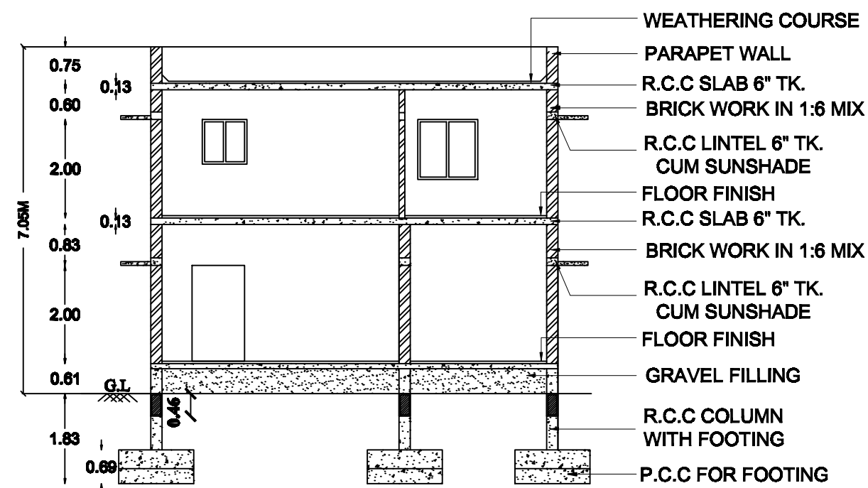
CROSS SECTION AT A-A
