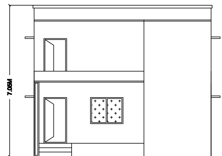
FORNT ELEVATION
