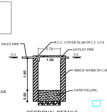
RAIN WATER COLLECTION PIT
