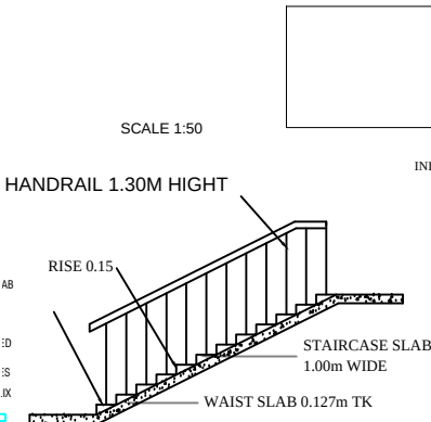
STAIRCASE DETAILS
