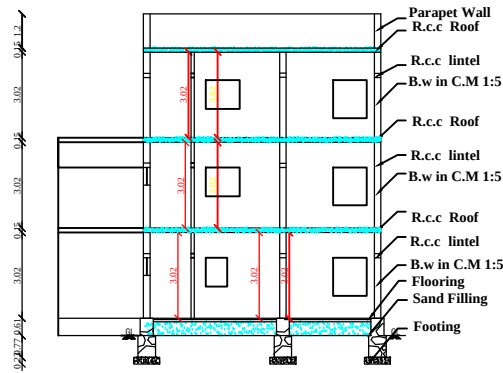
SECTION AB
