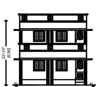
FRONT ELEVATION
