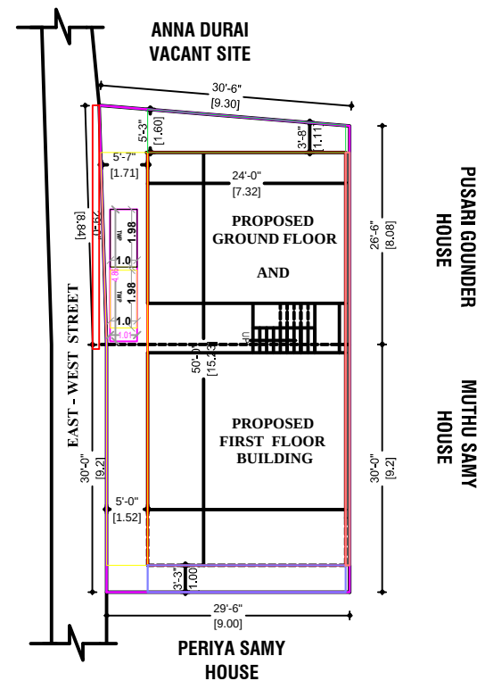
SITE PLAN
