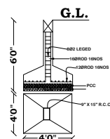
FOUNDATION DETAILS (NOT TO SCALE)
