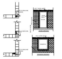
EARTHQUAKE SAFE DESIGN (NOT TO SCALE)
