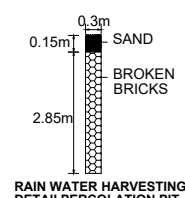
DETAIL PERCOLATION PIT (NTS)
