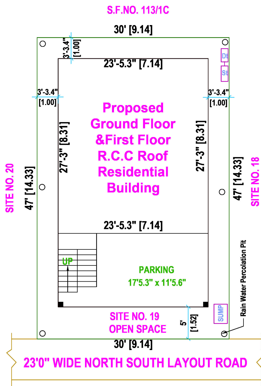
SITE PLAN SCALE 1" : 8' 0"
