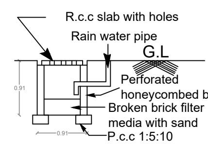
SECTION ON B1 B1
