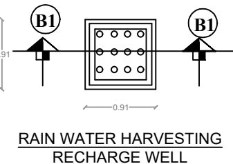
RAIN WATER HARVESTING RECHARGE WELL
